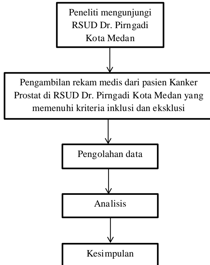
Gambar 3.1 Alur Penelitian
