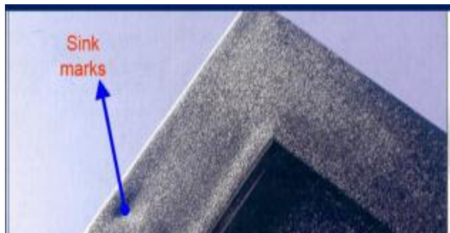
Gambar 2.5. Sink Marks ( https://tokoplas.com )
