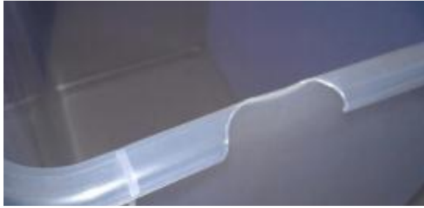
Gambar 2.3 Cacat Short Shot ( https://tokoplas.com )
