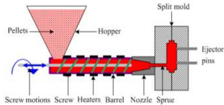
Gambar 2.1 Mesin Injection (Sumber google, 2016)
