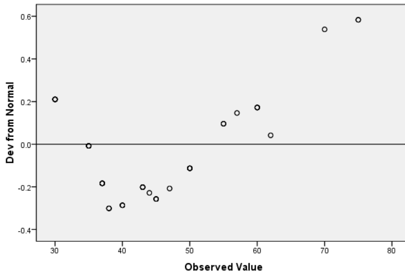
Detrended Normal Q-Q Plot of Pre Test
