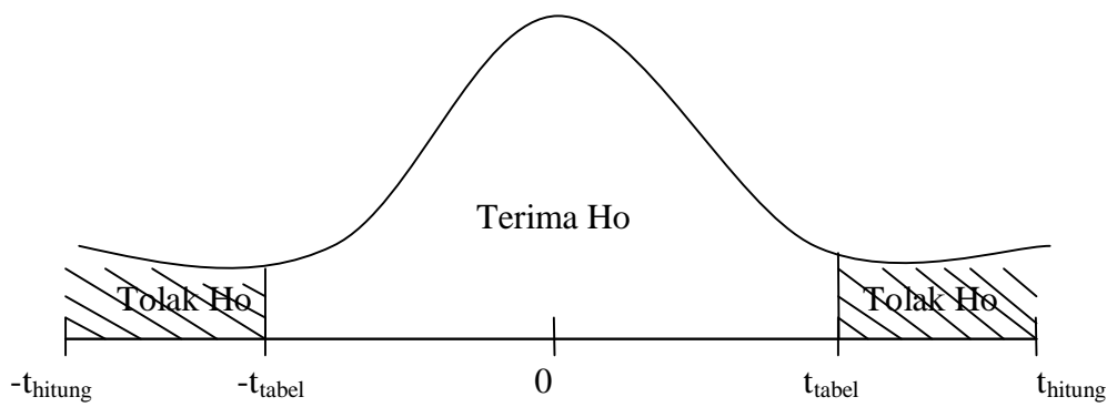
Gambar III.1 Kurva Distribusi Hipotesis
