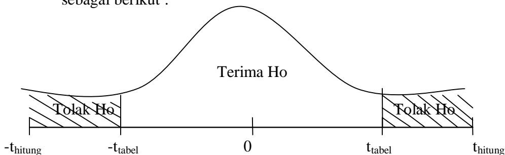
Gambar III.2 Kurva Distribusi Hipotesis
