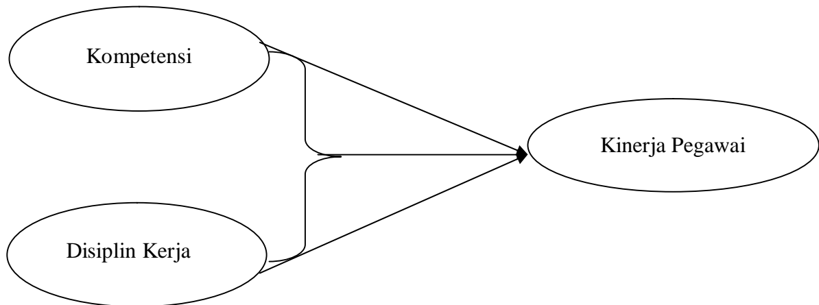
Gambar II.3 Paradigma Penelitian
