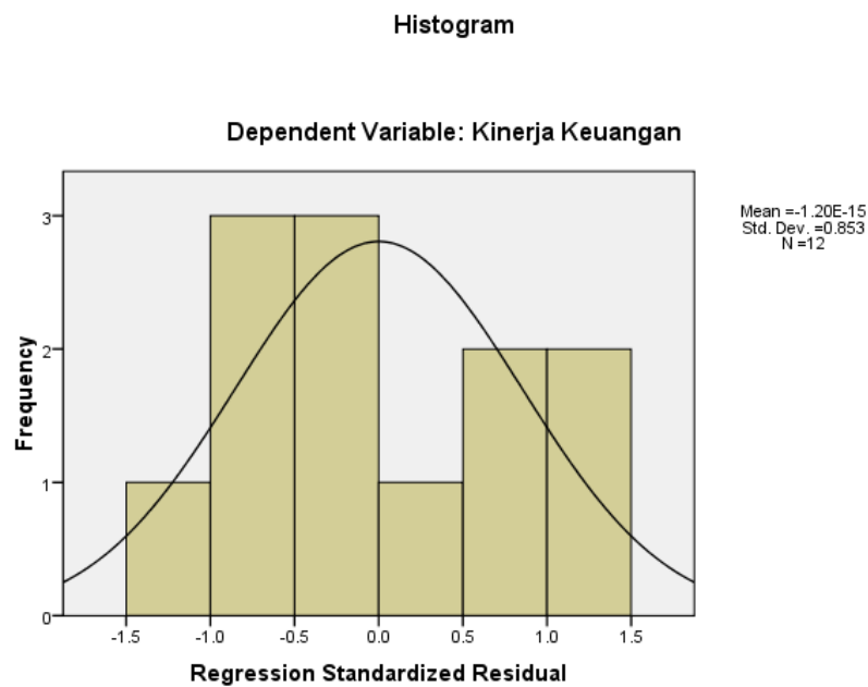
Gambar 4.2 Histogram normalitas
