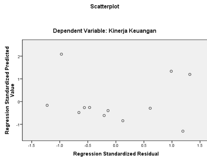
Gambar 4.3 Scatterplot
