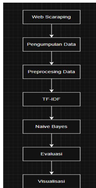
Gambar 3.1 Alur Penelitian
